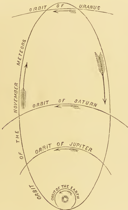
FIG. 106.—Orbit of November meteors.
